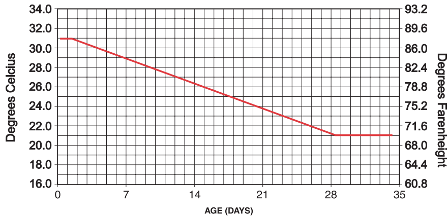
Brooding temperature profile for Cobb Avian 48 grandparent breeders
